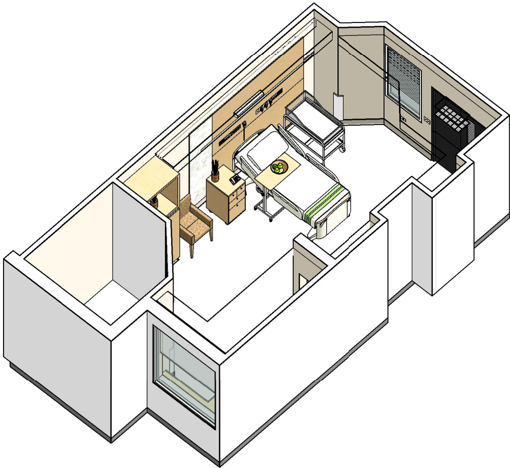
ISOMETRIC VIEW 01
